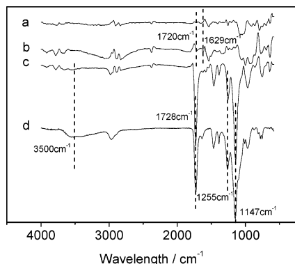
Figure 1. ATR-FTIR spectra of crude MWNTs (a), MWNTs-CH=CH 2 (b), MWNTs-MIPs (c), and pure MIPs (d).
