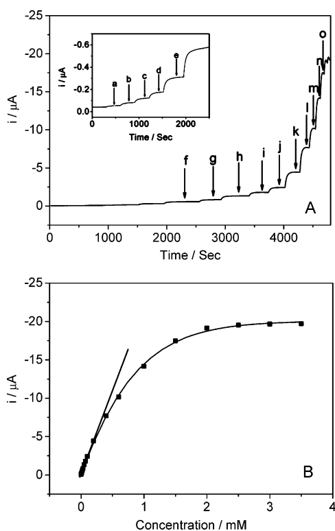
Figure 7. Typical current response curve at MWNTs-MIPs1 modified glassy carbon electrode with addition of increasing concentration of DA in PBS. Applied potential: +0.3V (A) and validation curve for DA obtained by I - T curve (B). Concentration of DA: 5.0 \times 10^{-7} (a), 1.5 \times 10^{-6} (b), 3.0 \times 10^{-6} (c), 5.0 \times 10^{-6} (d), 1.0 \times 10^{-5} (e), 2.0 \times 10^{-5} (f), 3.0 \times 10^{-5} (g), 5.0 \times 10^{-5} (h), 7.0 \times 10^{-5} (i), 1.0 \times 10^{-4} (j), 2.0 \times 10^{-4} (k), 4.0 \times 10^{-4} (l), 6.0 \times 10^{-4} (m), 1.0 \times 10^{-3} (n), and 1.5 \times 10^{-3} mol/L (o).
