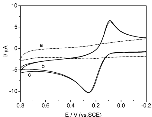
Figure 6. Cyclic voltammograms of modified electrode in fresh PBS buffer solution after the modified electrodes were incubated in 1.0 \times 10^{-4} mol/L AA (a), 1.0 \times 10^{-4} mol/L DA (b), and mixed solution of 1.0 \times 10^{-4} mol/L DA and 1.0 \times 10^{-4} mol/L AA (c) for 10 min.
