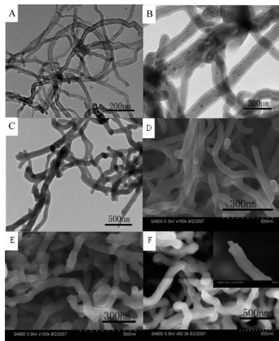
Figure 3. TEM of MWNTs (A), MWNTs-MIPs1 (B), and MWNTs-MIPs2 (C); SEM of MWNTs (D), MWNTs-MIPs1 (E), and MWNTs-MIPs2 (F).
