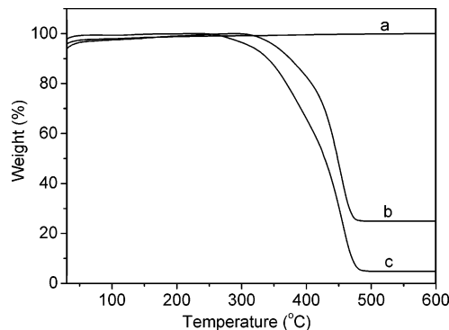
Figure 2. TGA at a heating rate of 20^\circ\text{C min}^{-1} from room temperature to 600^\circ\text{C} under a N 2 atmosphere for crude MWNTs (a), MWNTs-MIPs1 (b), and pure MIPs (c).
