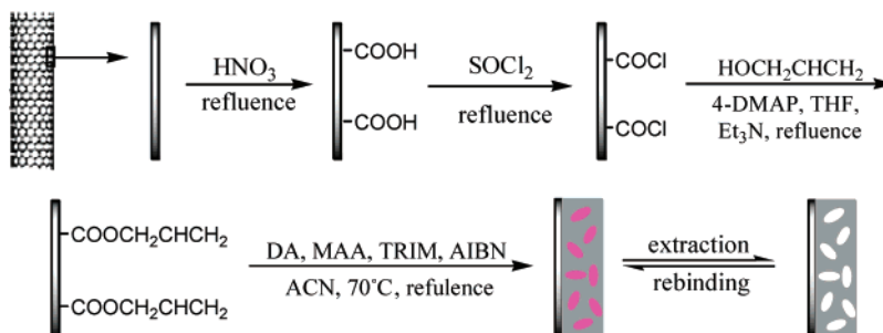
SCHEME 1: Synthesis Route of MWNTs-MIPs
