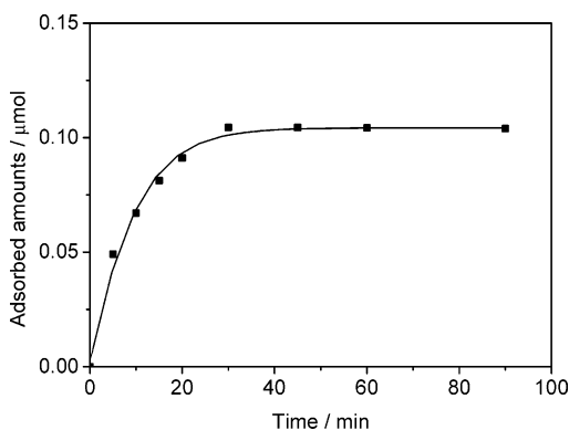
Figure 4. Curve of adsorption dynamics of DA to MWNTs-MIPs1. Amount of polymer, 5 mg; volume, 2.0 mL; initial concentration of DA, 0.2 mmol/L.
