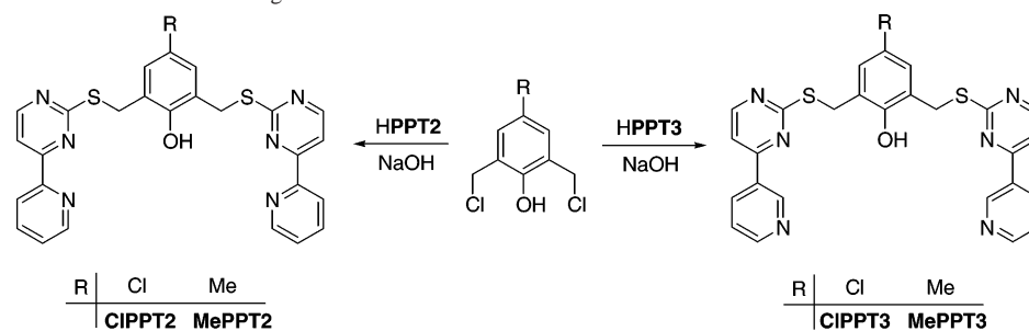
Scheme 1. Synthetic Methods for Thioether Ligands
