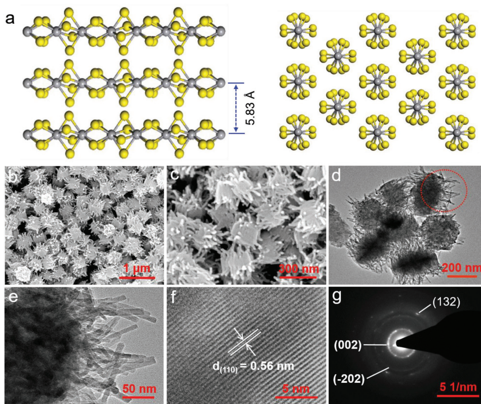
Figure 1. Schematic geometries of \text{VS}_4 and morphology characterizations of \text{VS}_4 nanodendrites. a) Lateral-view (left) and vertical-view (right) of the “linear-chain” crystalline structure of \text{VS}_4 , showing an interval of 5.83 Å between the atomic chains. b–g) Morphology characterizations of \text{VS}_4 nanodendrites: b,c) SEM images, d,e) TEM images, f) HRTEM image, g) SAED pattern of \text{VS}_4 nanodendrites.
