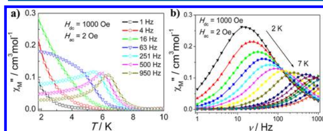
Figure 3. Variable-temperature (a) and variable-frequency (b) out-of-phase ac magnetic susceptibility data for 1 in a 1000 Oe dc field.
