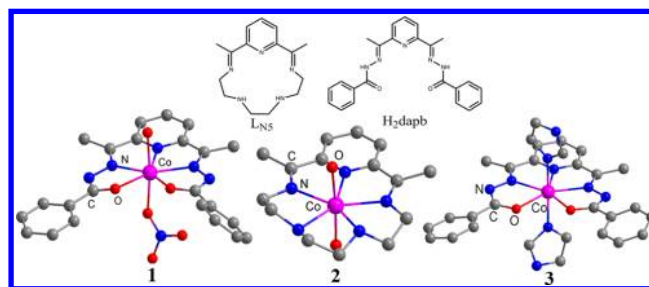
Figure 1. Structures of L_{NS} and H_2dapb ligands and Co II 1 – 3 . Hydrogen atoms are omitted for clarity.
