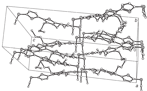
Figure 3. Perspective view of the packing structure of 2 with the unit cell; hydrogen atoms are omitted for clarity.
